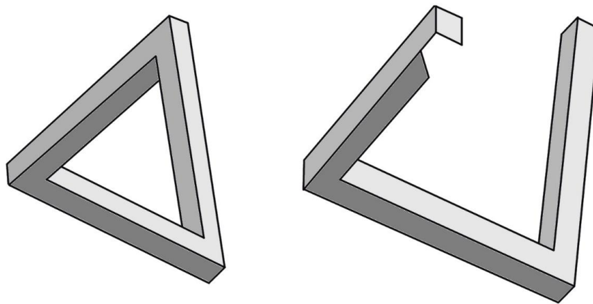
Figure 1: The Penrose triangle and the Gregundrum
